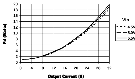
Power Dissipation vs Output Current (@Vout=+3.3V)
